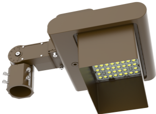
LF-SHROUD-D FULL-GLARE SHROUD CAN BE PAINTED 6 1/4" x 10 5/8" x 4 3/4"
