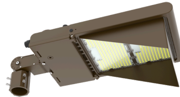
LF-SHROUD-B HALF SHROUD REVERSIBLE / CAN BE PAINTED 5 3/4" x 6" x 2"
