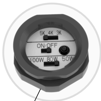
Pre-Installed Photocell with ON/OFF Switch
